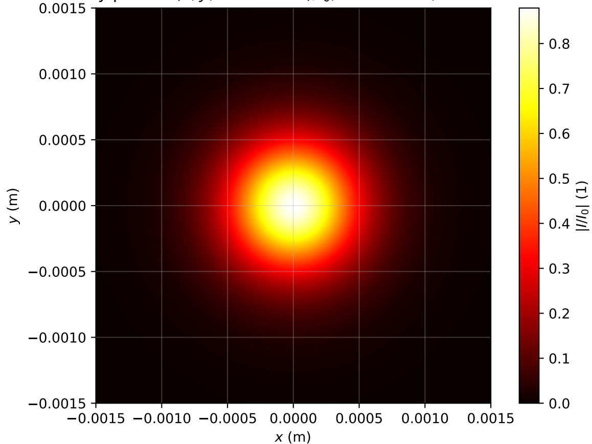
Intensity profile I(x, y, z = 2.229m)/I_0 , Pin=0.6Pcr, artificial time
